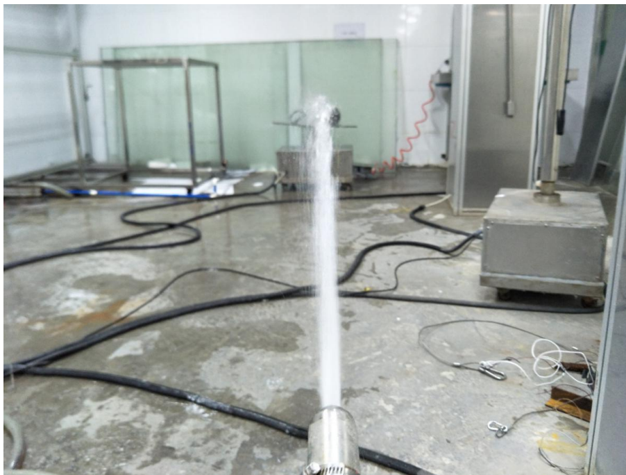
Photo 3: IPX6 test of model BL-D150-1204A
